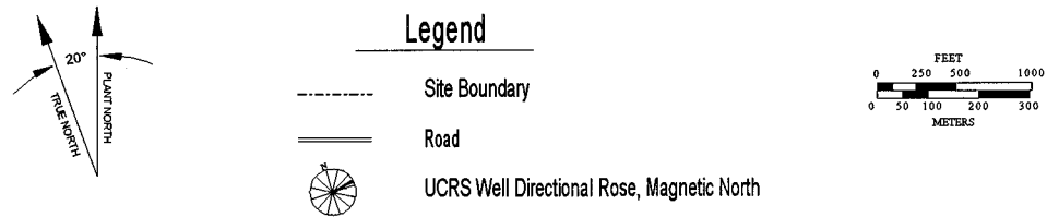
Figure 6. Map showing flow directions based on Colloidal Borescope measurements.
