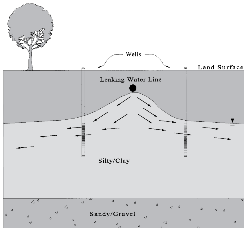
Figure 4. Conceptual illustration of the flow systems.
